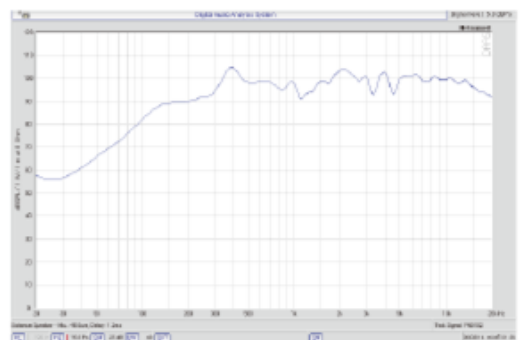
Frequency Response Curve
